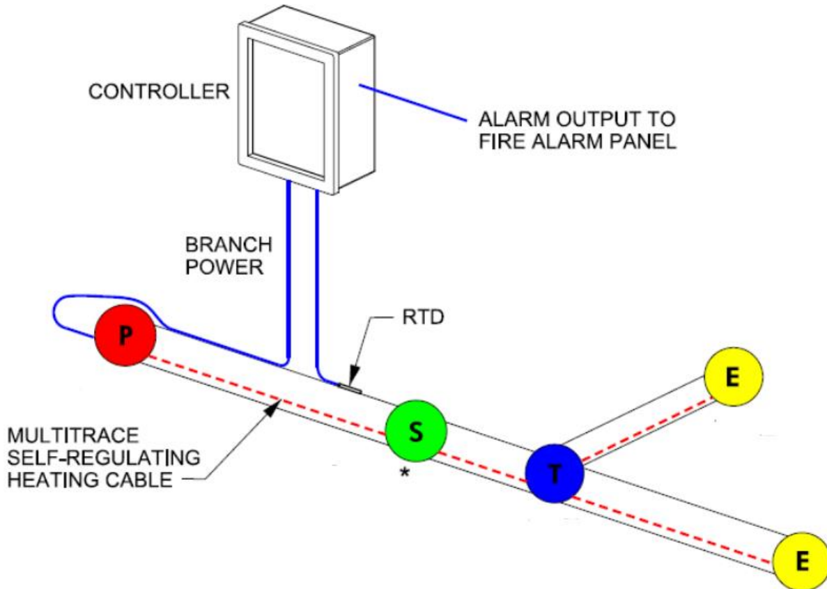
FIG. 2 – ABOVE GROUND SUPPLY PIPING
